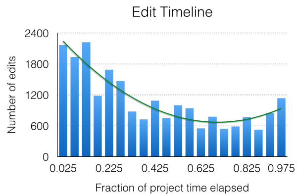
Figure 3: Editing timeline
